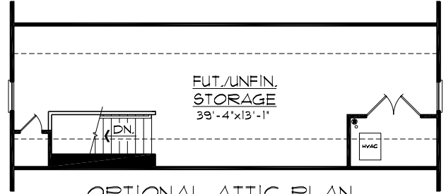
OPTIONAL ATTIC PLAN
