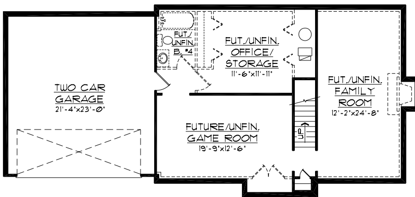
FOUNDATION PLAN
